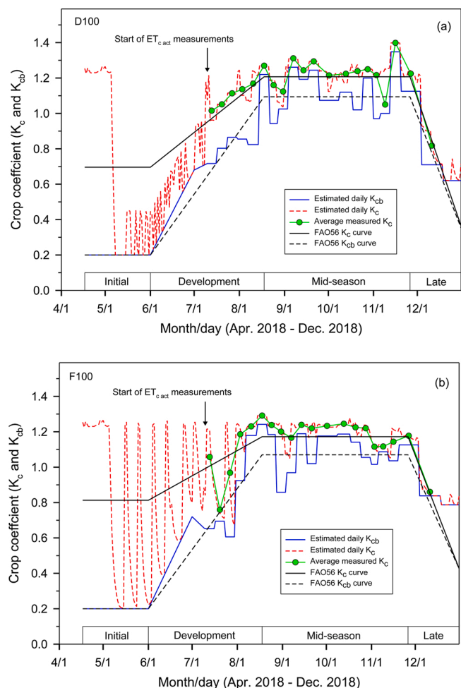
Fig. 6. Estimated daily basal ( K_{cb} ), single ( K_c ) crop coefficients, average measured ( K_c ), and standardized FAO56 curves for 2018 (1st year) guayule at Eloy for the (a) D100 and (b) F100 treatments.
