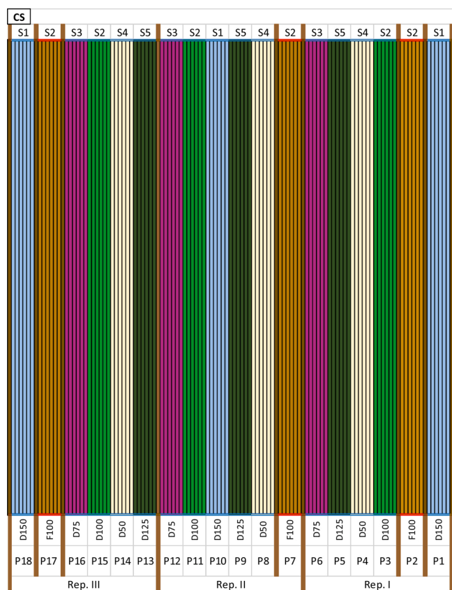
Fig. 1. Layout of the irrigation experiment. The fields at Maricopa and Eloy were divided into three blocks (Reps. I-III). Irrigation treatments (D50-D150, F100) were distributed randomly inside each block, which resulted in 18 plots (P1-P18). The control station (CS) of the subsurface drip system was located at the NE corner of the field.
